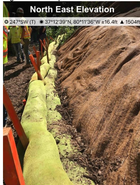
Fig. 2. ECD's in place at intersection of ROW and AR278.01
