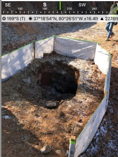
Fig. 1 St#11427+00 soil pipe protected by P1 fence
