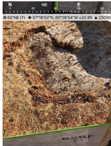
Fig. 4 St#11361+00 sump end treatment is undermined
