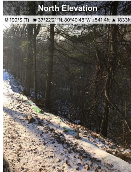
Fig. 2 ECD's in place on AR GI 234
