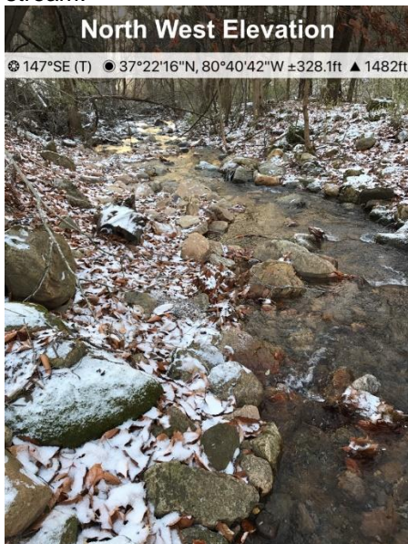
Fig. 3 Designated stream SQ 14 has signs of road gravel in stream.
