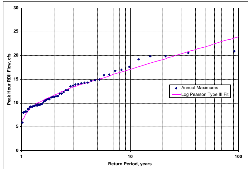
Figure 6-6. Example of Probability Plot
