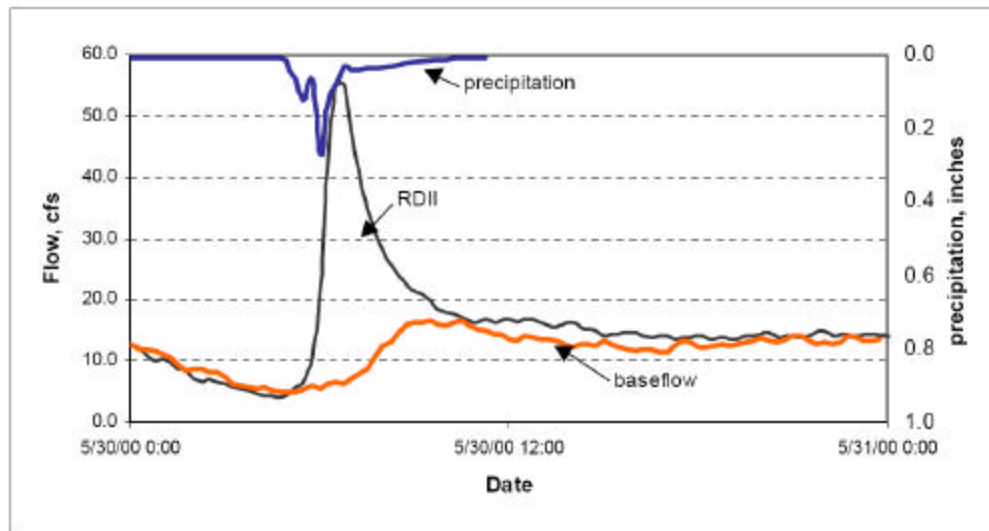
Figure 6-2. Components of Sewer Flow
