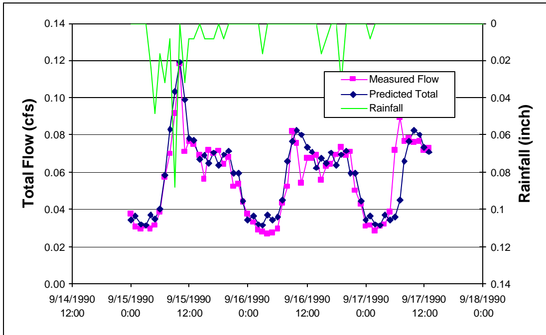
Figure 6-5. Modeled Versus Observed Flow
