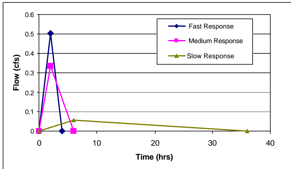
Figure 6-4. Synthetic Unit Hydrographs
