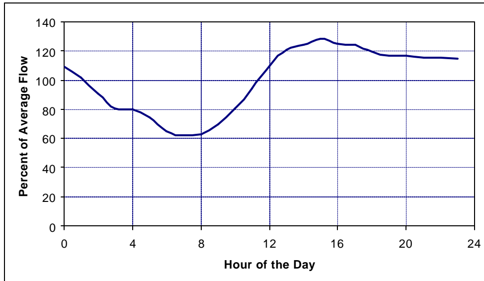
Figure 6-3. Example Diurnal Curve
