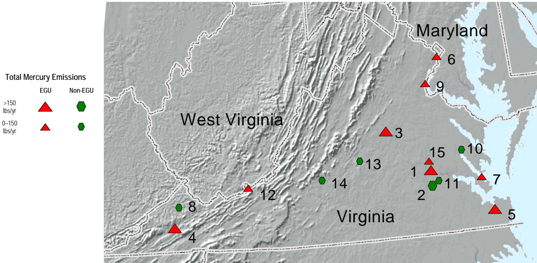
Figure 3-1. Location and Magnitude of the Top 15 Virginia Mercury EGU and Non-EGU Point Sources for 2022 (Hg-Total Mercury)
