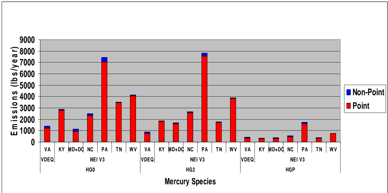
Figure 2-2. Comparison of the 2002 VDEQ Speciated Mercury Emissions Inventory with the 2002 NEI Version 3 Inventory for Selected Neighboring States
